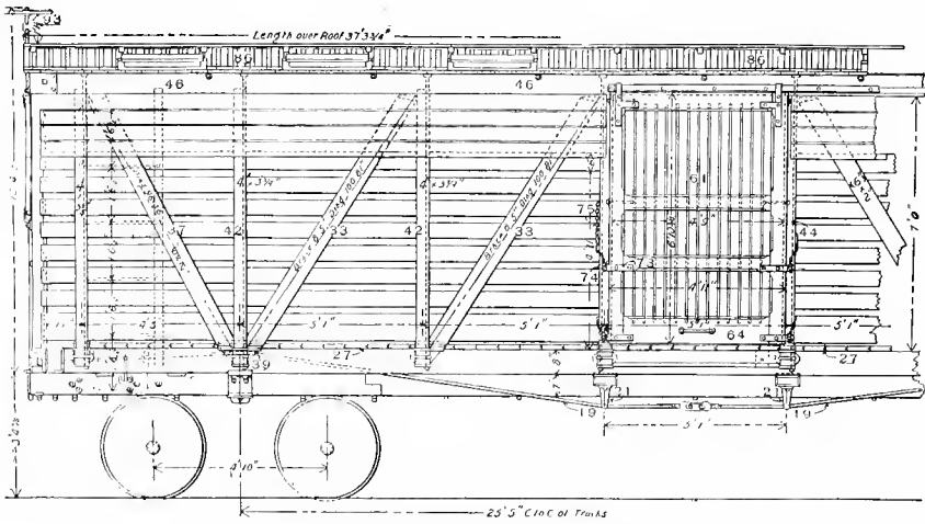
Fig. 369. Part Side Elevation.
